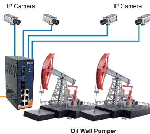
Connections of Ethernet devices
