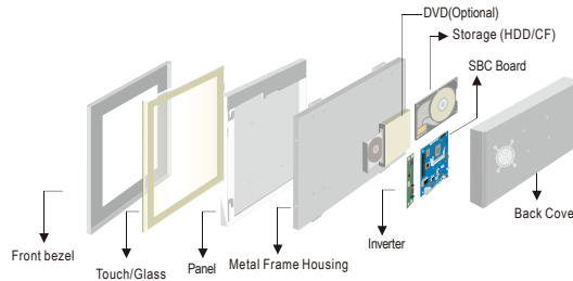
Mechanical design
